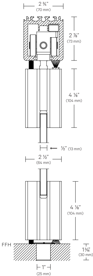
Head Track with Concealed Locking and Floor Socket
