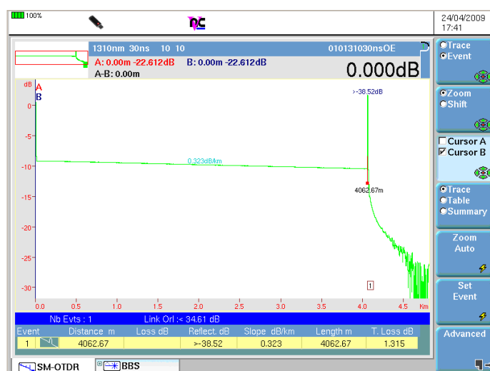
Figure 12. Feeder or distribution cable test only
