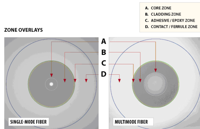
Figure 2. Fiber connector end face inspection zones
