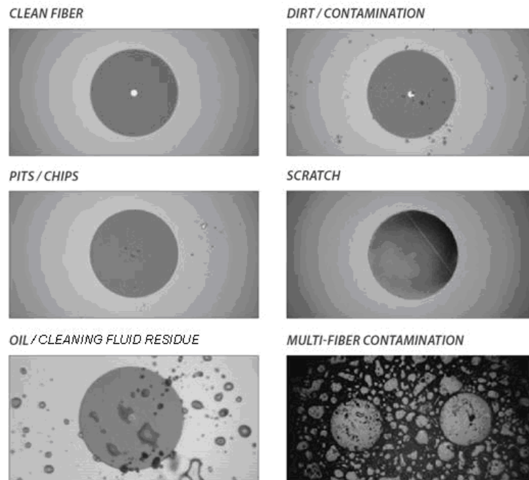
Figure 3. Fiber connections and various connector end face views as seen through an inspection scope
