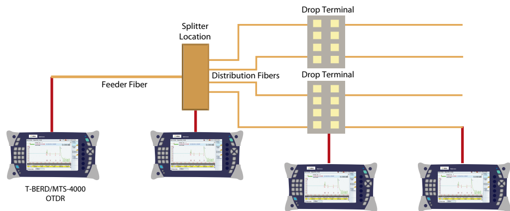
Figure 1. Possible access points for FTTH network qualification
