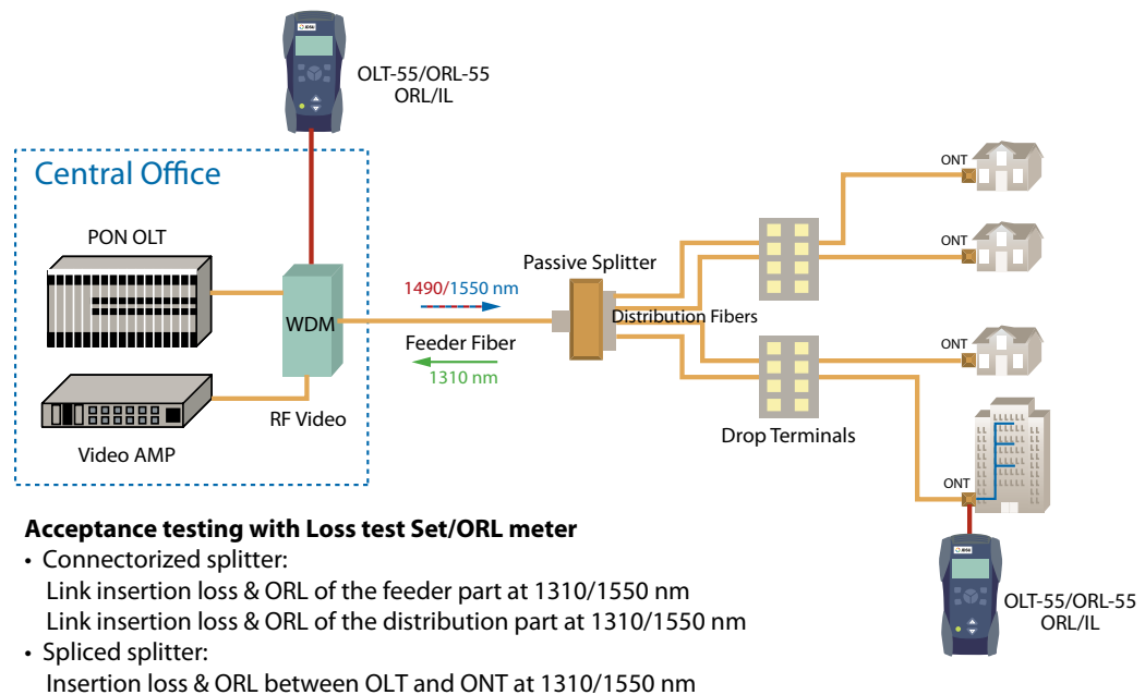
Figure 17. Qualifying the FTTH network with a loss test set/ORL meter
