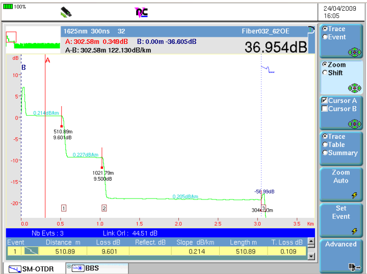
Figure 14. Cascaded splitter network test from ONT, without launch cable
