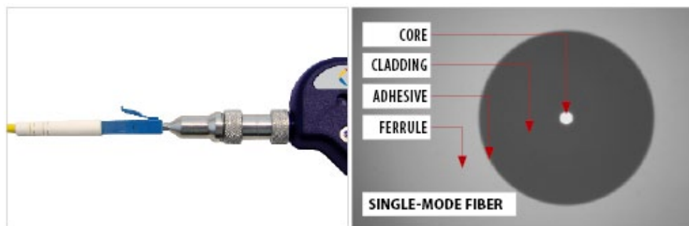
Figure 6. Patchcord microscope inspection
