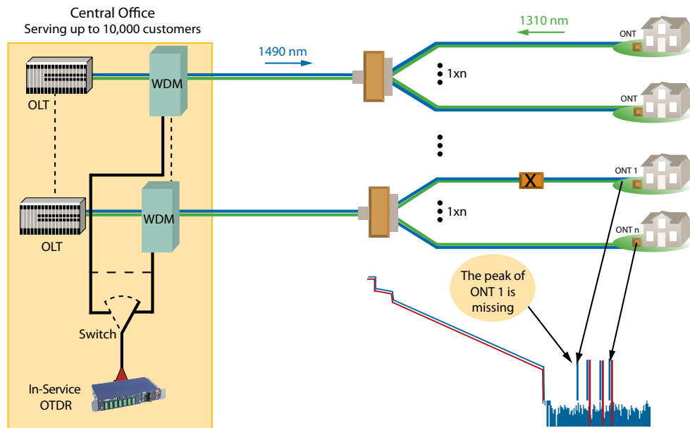
Figure 20. FTTH network monitoring tools
