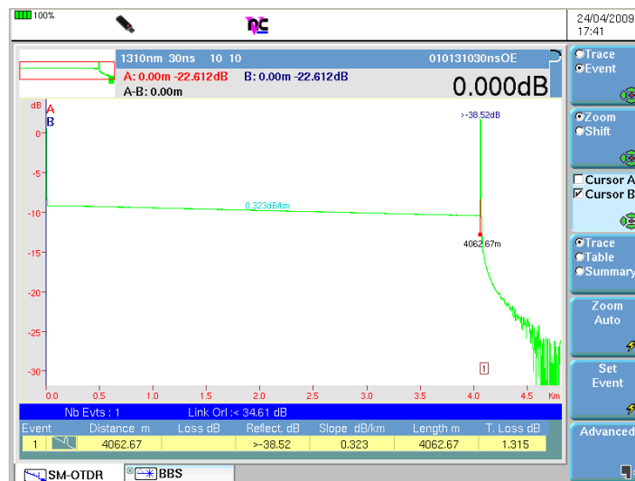
Figure 13. Distribution test only from ONT to first splitter, without launch cable
